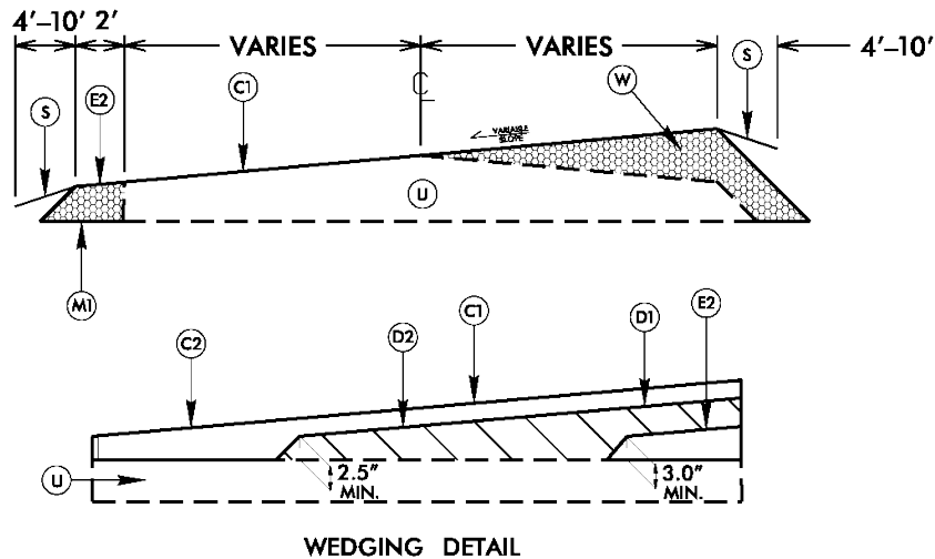
WEDGING DETAIL
